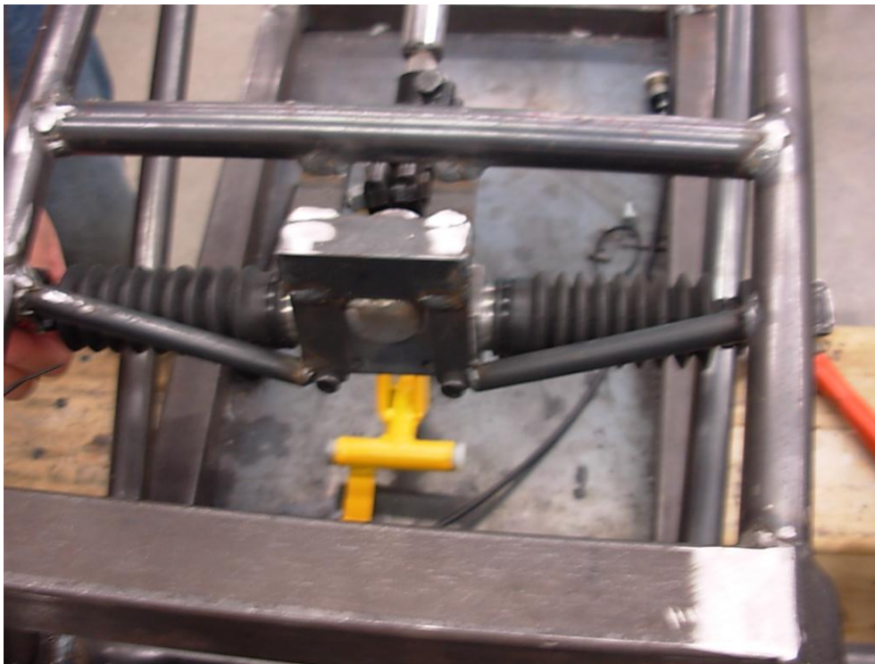
The steering rack also is the mount for our brake and gas pedals.
